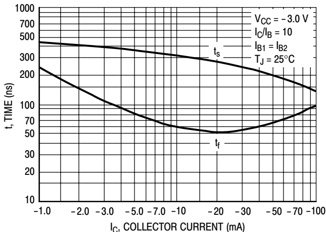
Figure 11. Turn-Off Time
